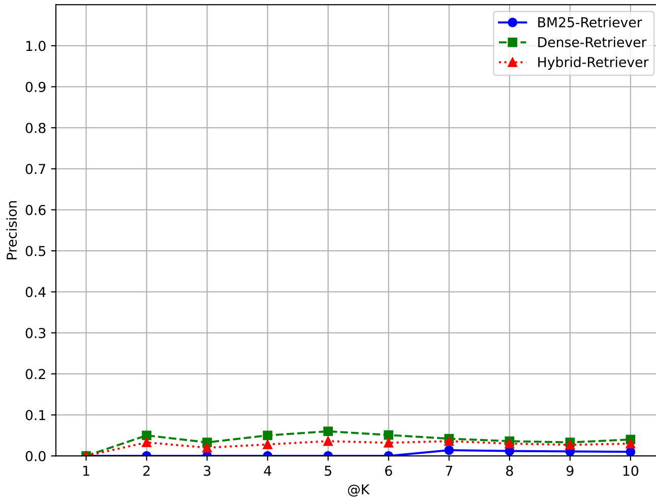
Query 44
